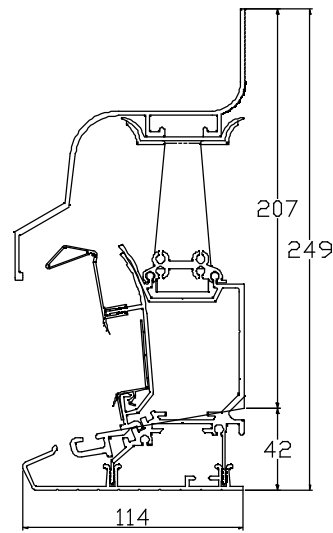
10 DEGREE HALF RIDGE
