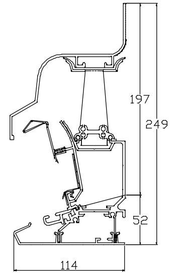
15 DEGREE HALF RIDGE
