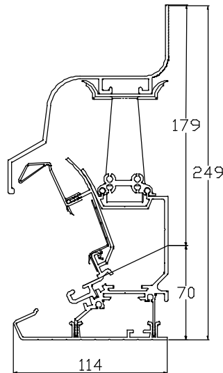
25 DEGREE HALF RIDGE
