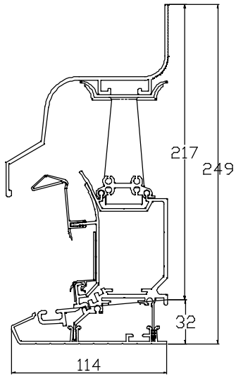
5 DEGREE HALF RIDGE
