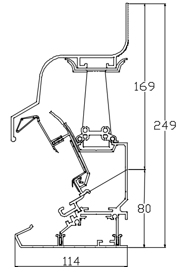
30 DEGREE HALF RIDGE
